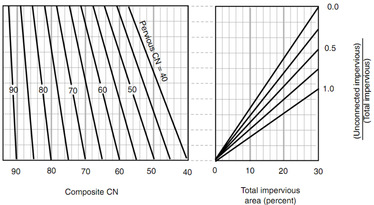
Composite Curve Number with Unconnected Impervious Area
