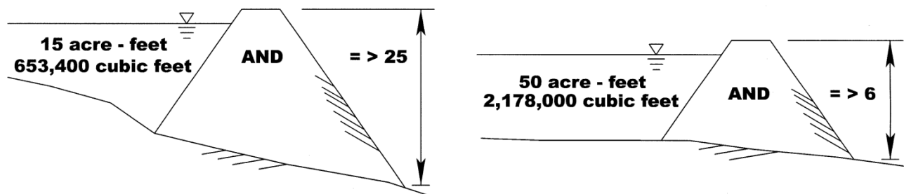
Figure 9-1 Embankment Rule Classifications
