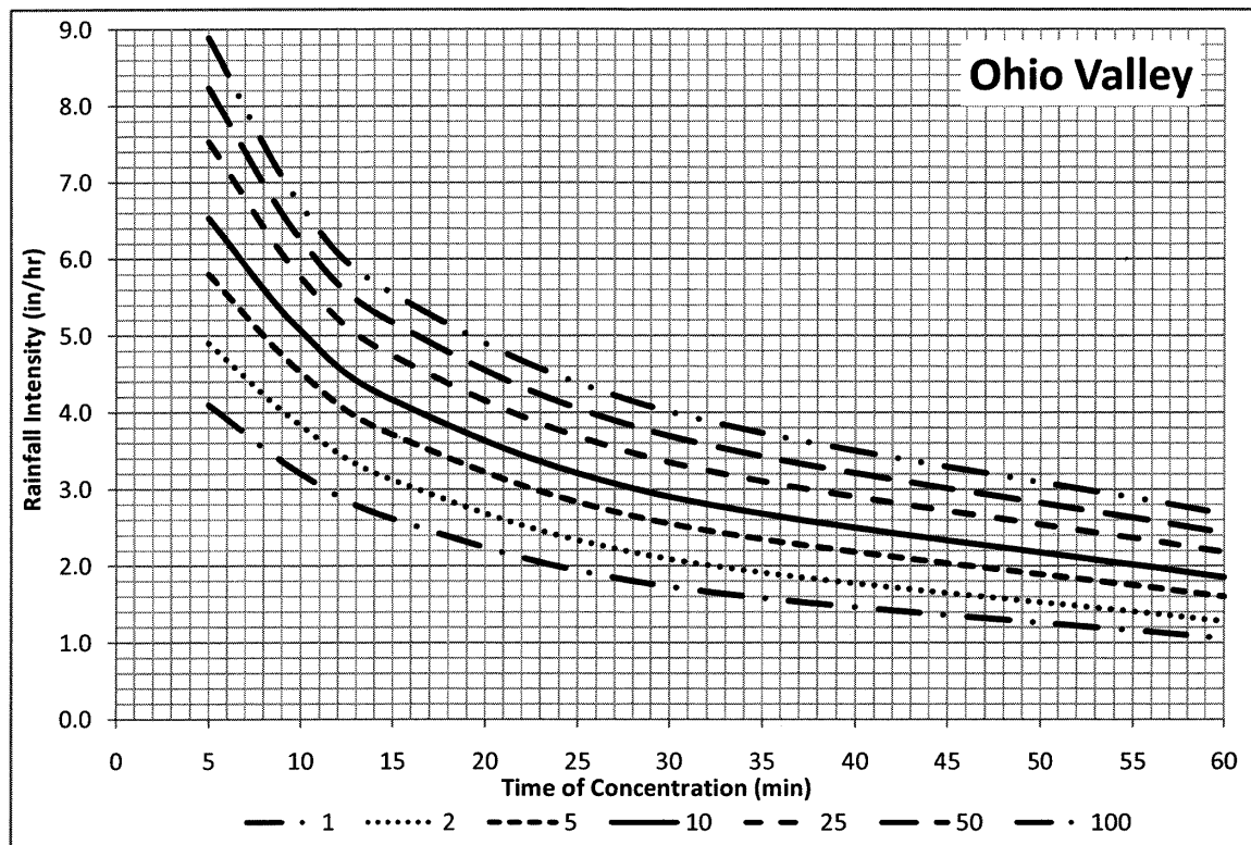
Chart 4-2 Intensity-Duration-Frequency Curves for West Virginia
