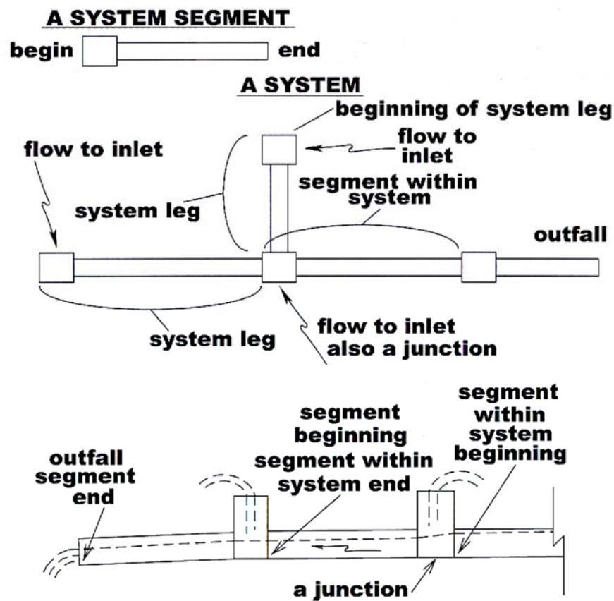
Figure 5-7 Hydraulic Design
