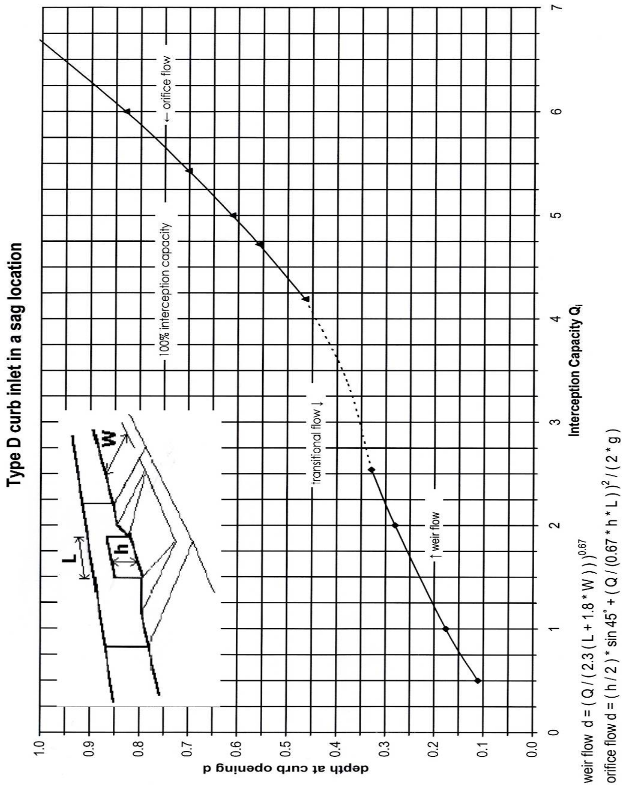
Chart 5-22 Type D Curb-Opening Inlet in a Sag Location
