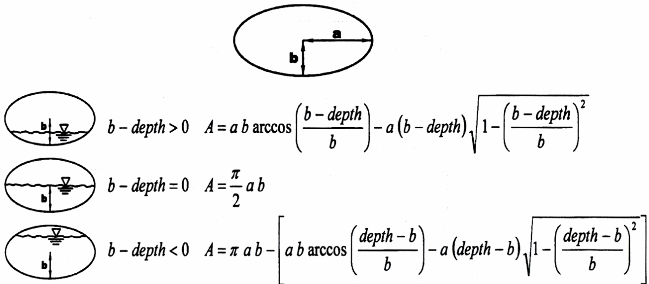
Figure 8-9 Elliptical Pipe Flow Area
