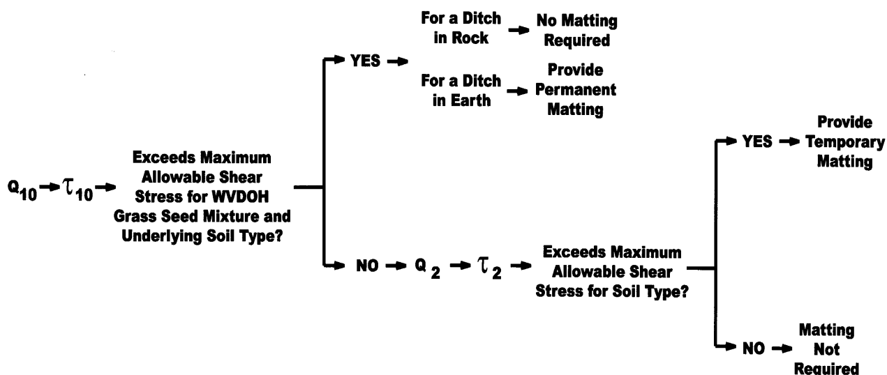
Figure 6-1 Ditch Analysis Flowchart
