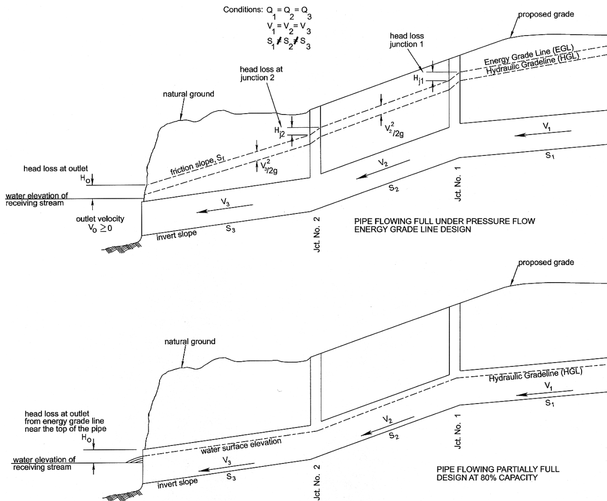
Figure 5-8 Energy Losses in a Storm Drain System
