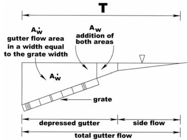
Figure 5-2 Flow Area Ratio Grate Width Less Than Gutter Width
