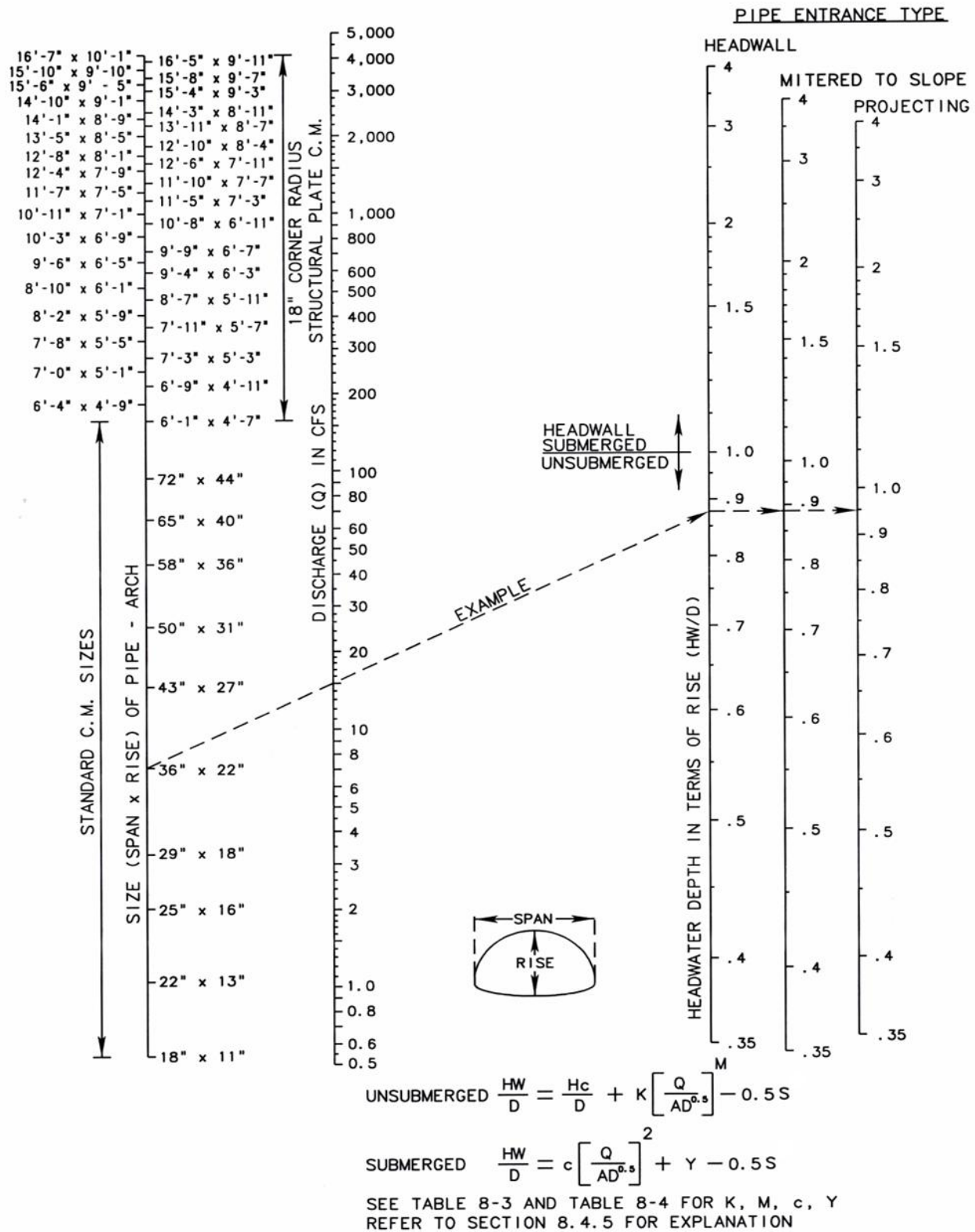
Chart 8-19 Standard C.M. Pipe Arch Culverts with Inlet Control
