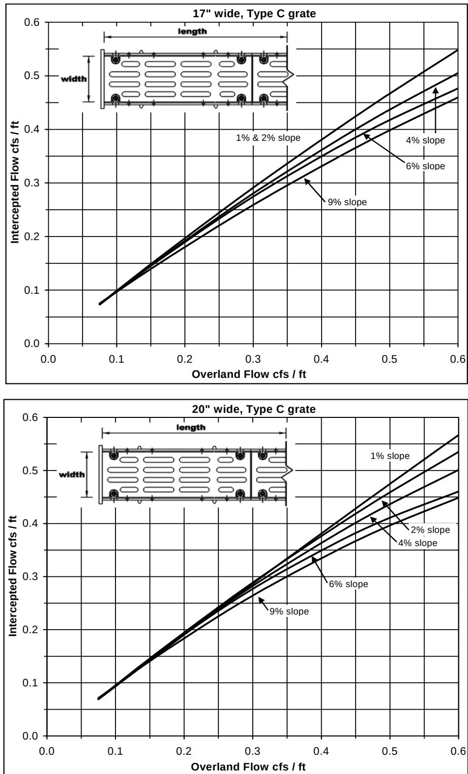
Chart 5-16 Concrete Box with Type C Grate (17", 20")
