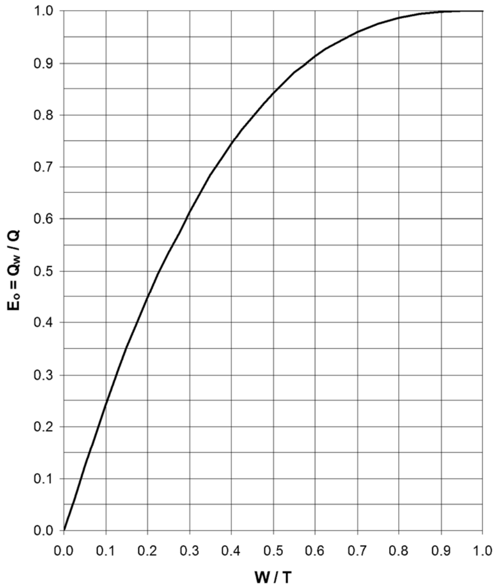
Chart 5-3 Ratio of Frontal Flow to Total Gutter Flow for A Uniform Cross Slope
