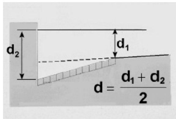
Figure 5-5 Average Depth Over a Grate
