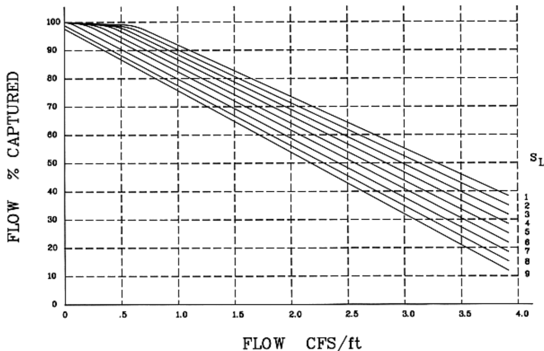
Chart 5-18 Concrete Box with Vane Style Grate (14")
