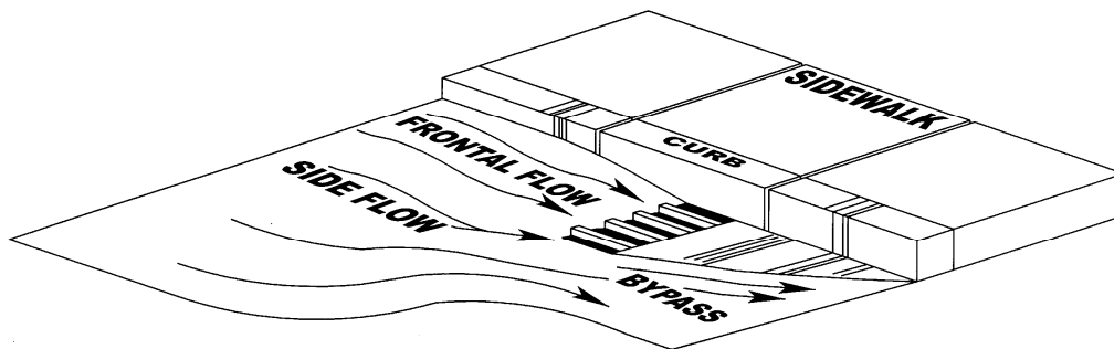
Figure 5-3 Intercepted Flow with Bypass
