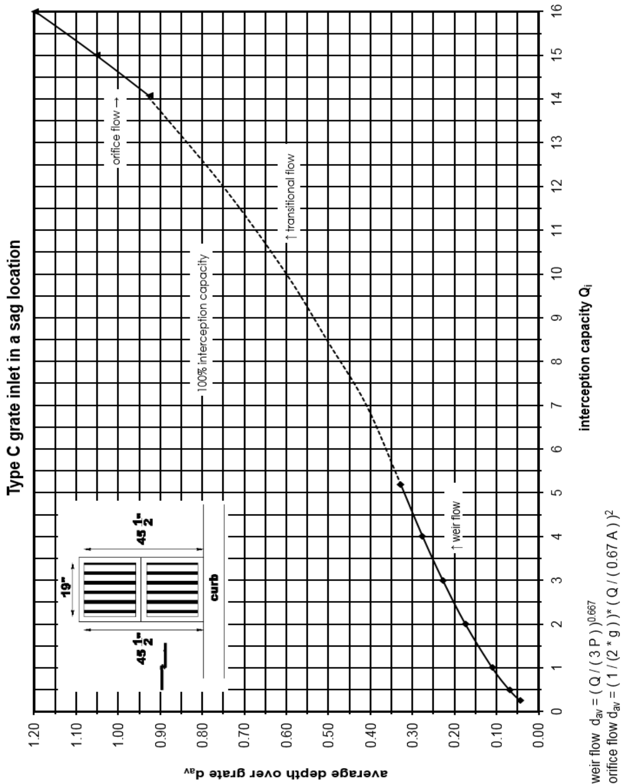
Chart 5-21 Type C Grate Inlet in a Sag Location
