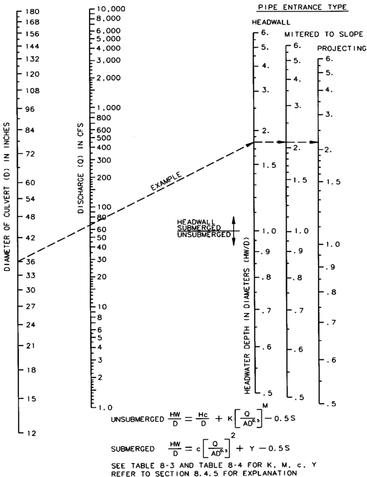
Chart 8-6 HDPE Pipe Culverts with Inlet Control
