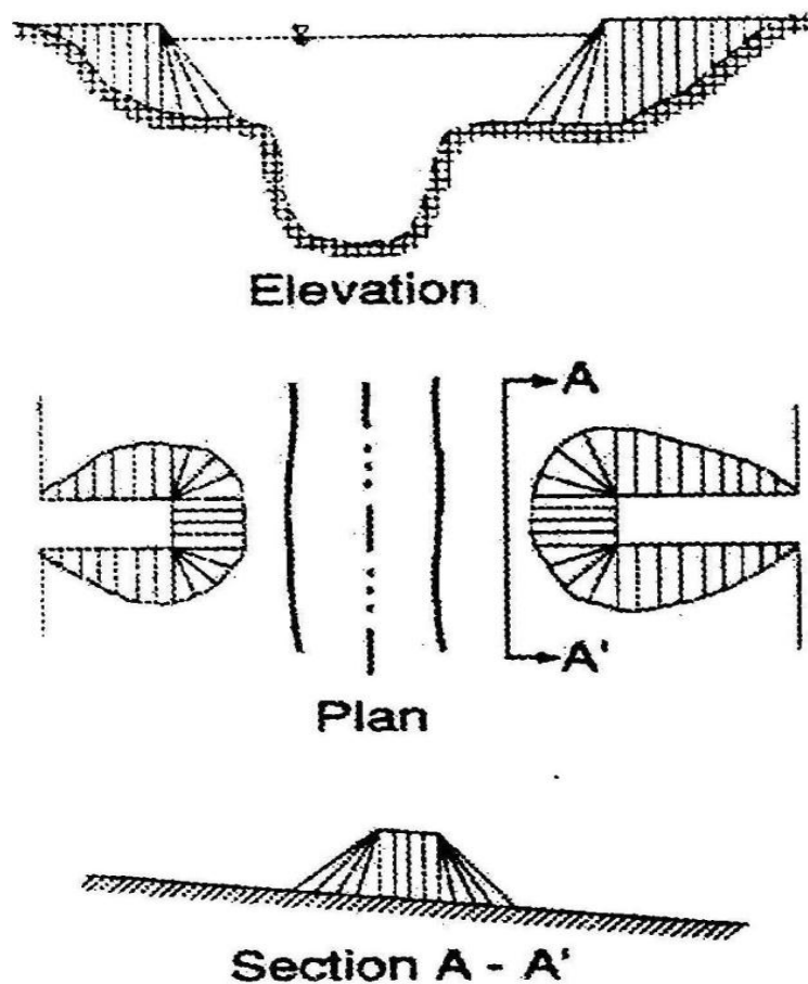
Figure 10-5 Spill-Through Abutment
