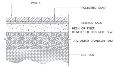
Typical Paver Detail
