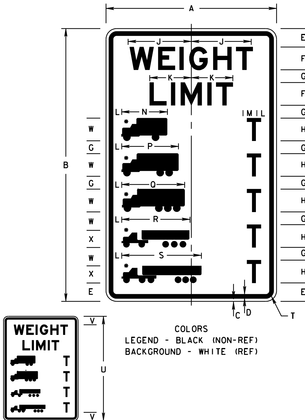
DIMENSIONS (INCHES)
