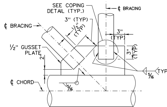
DETAIL 4
