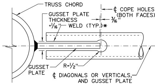
COPING DETAIL
