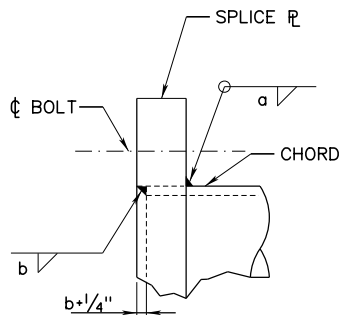
DETAIL 7
