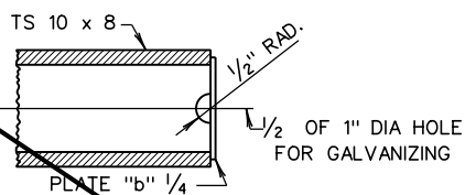
DETAIL E
