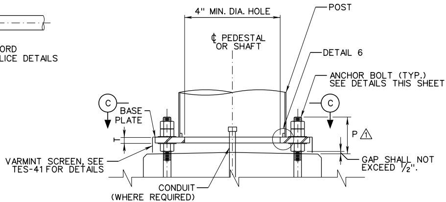
DETAIL 5
