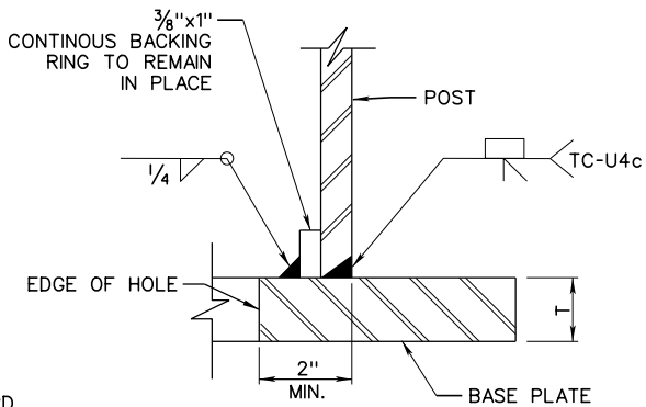
DETAIL 6
