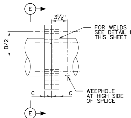
DETAIL 3
