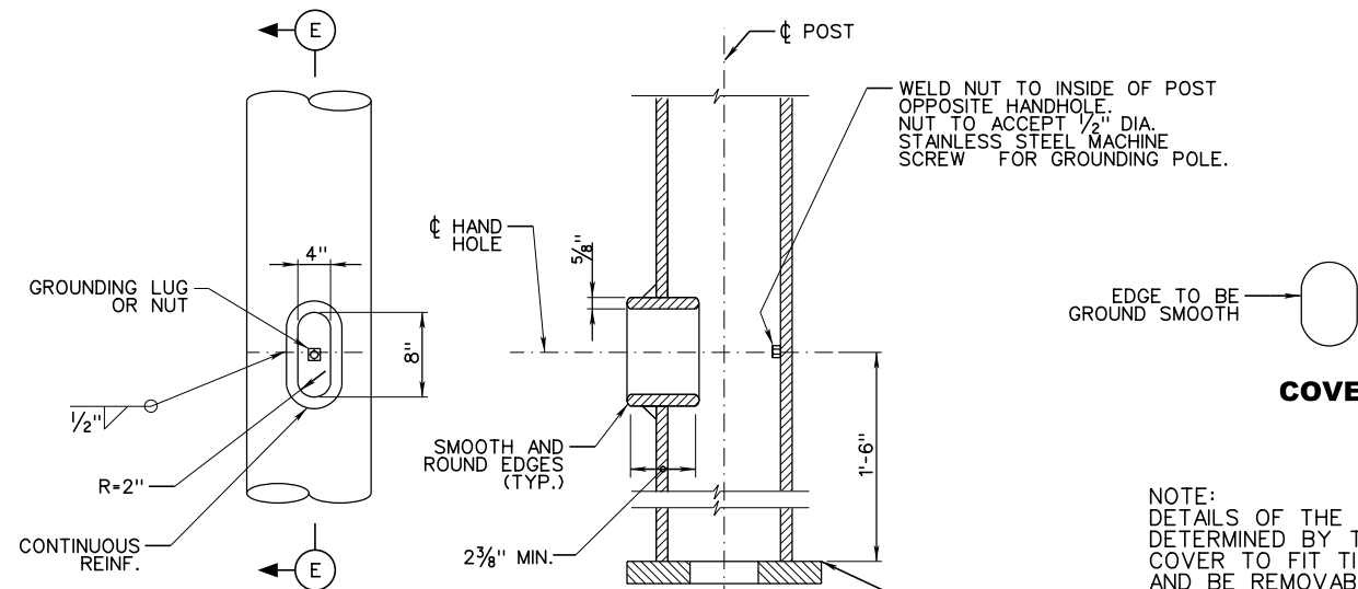
SECTION E-E PLATE POST HANDHOLE DETAIL
