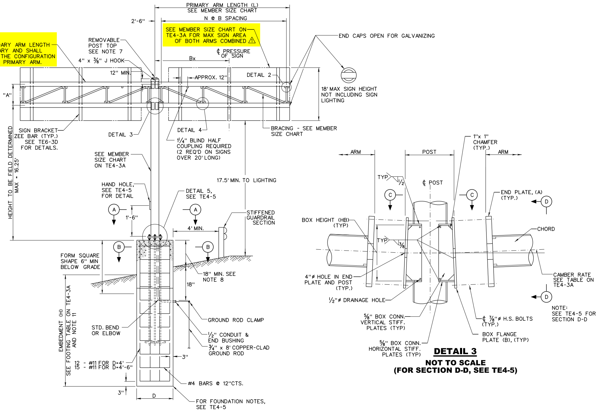
ELEVATION SEE NOTE 2
