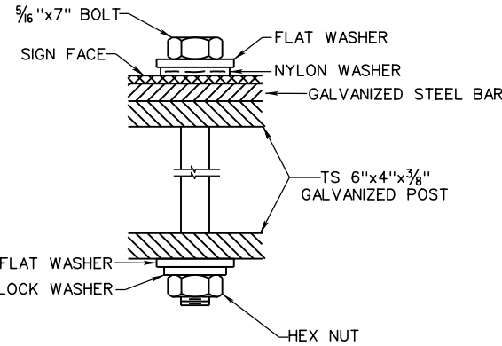
DETAIL 'C'
