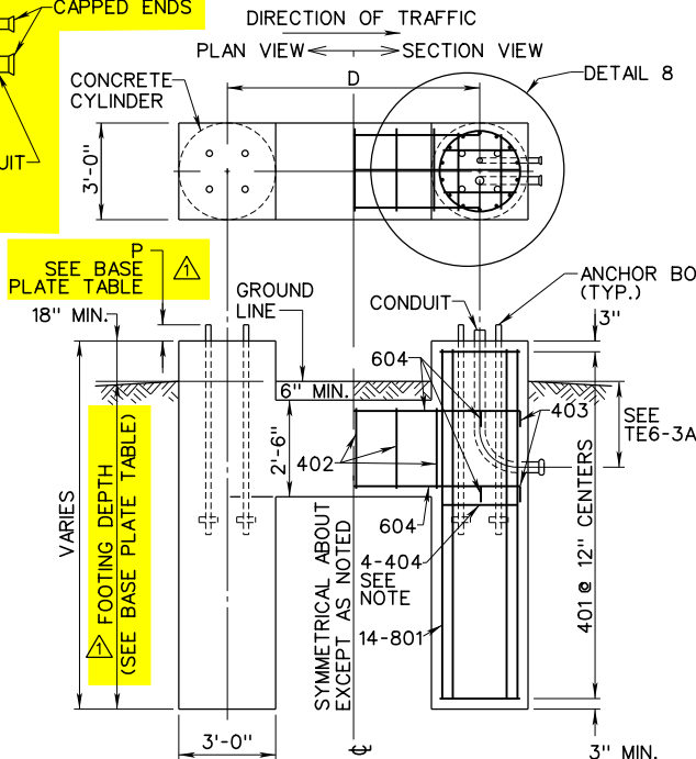
FOUNDATION DETAIL
