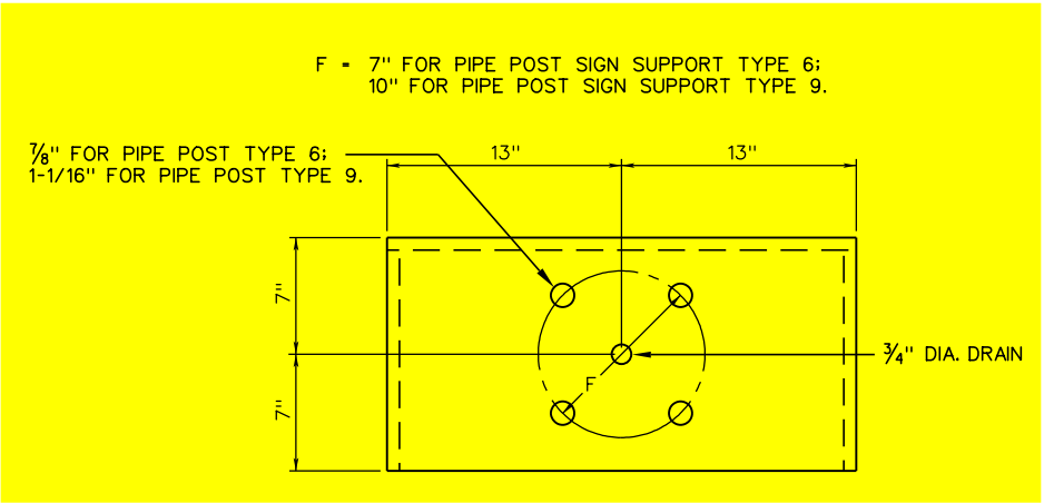
BRACKET TOP VIEW
