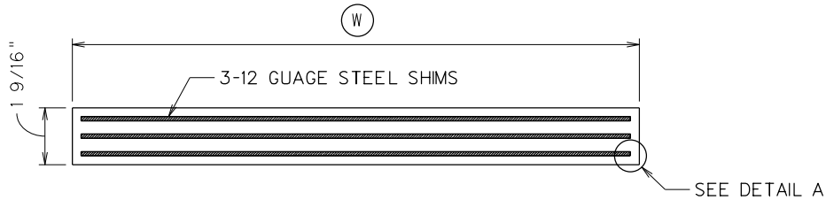
TYPICAL SECTION - TYPE A1
