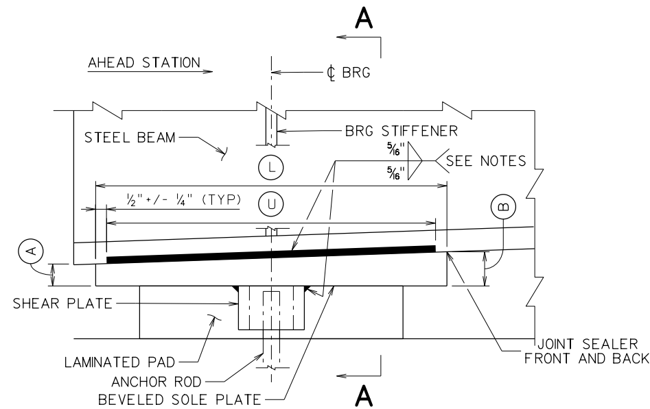
FIXED SIDE ELEVATION (SLOPES > 0.50% ALONG BEAM)
