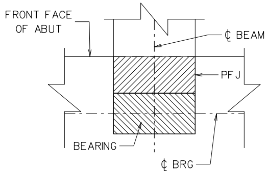
BEARING LAYOUT
