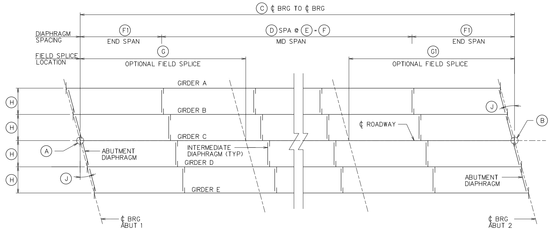
FRAMING PLAN
