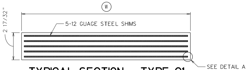
TYPICAL SECTION - TYPE C1
