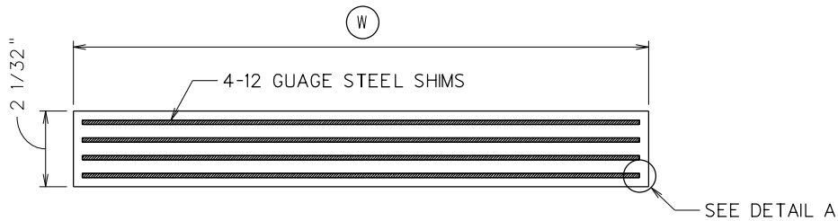
TYPICAL SECTION - TYPE B1
