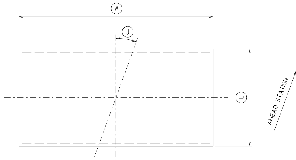
BEARING PLAN
