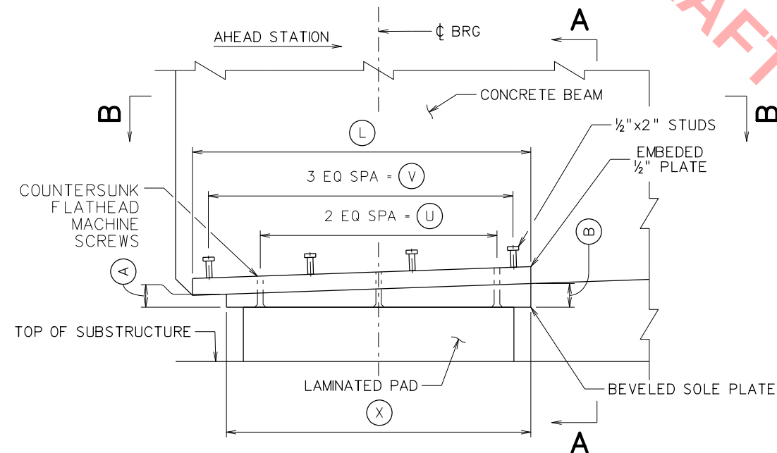
NON-GUIDED SIDE ELEVATION (SLOPES > 2.00% ALONG BEAM)
