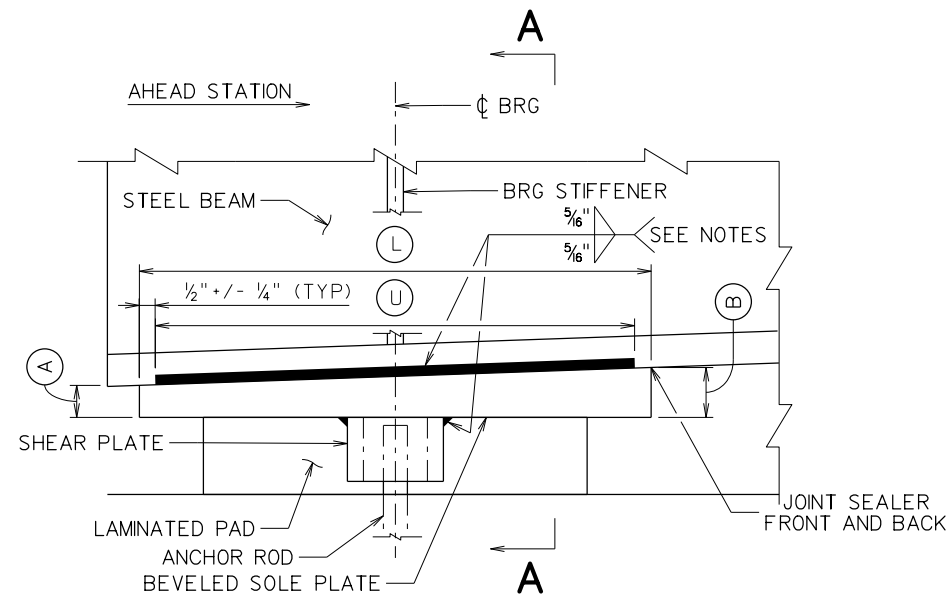
GUIDED SIDE ELEVATION (SLOPES > 0.50% ALONG BEAM)
