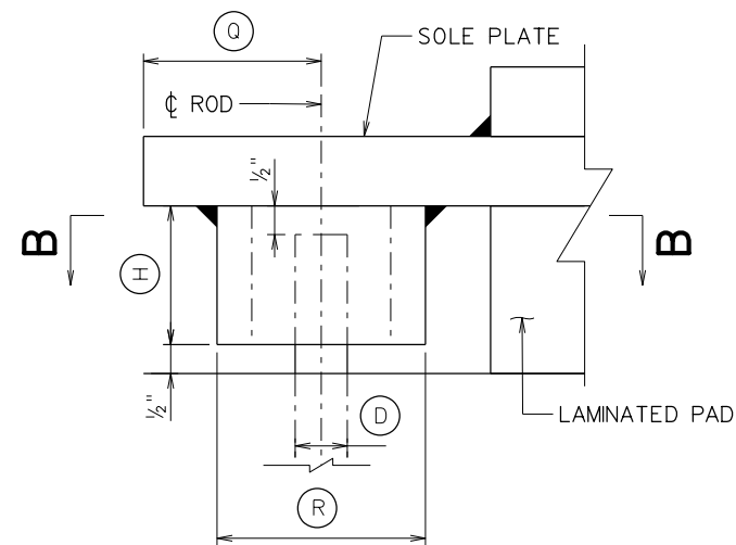
SHEAR KEY DETAIL
