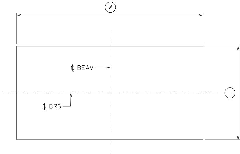
BEARING PLAN
