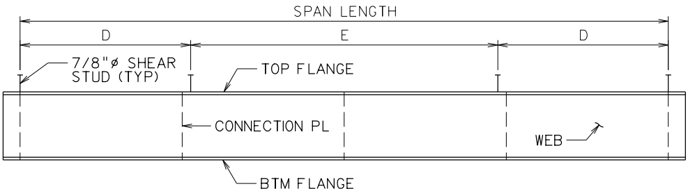
BEAM ELEVATION
