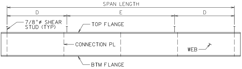
BEAM ELEVATION
