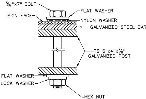
DETAIL 'C'
