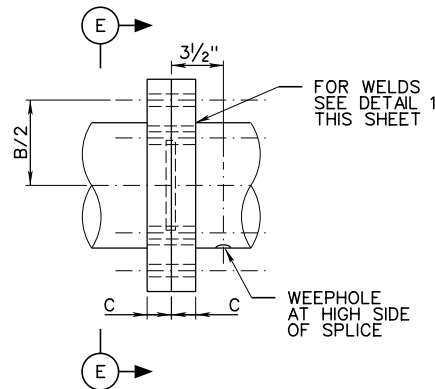
DETAIL 3
