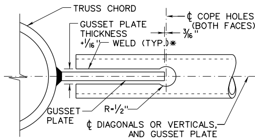
COPING DETAIL
