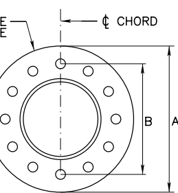
SECTION E-E SEE NOTE 4
