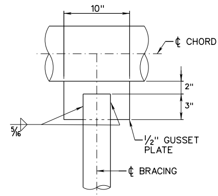
DETAIL 2
