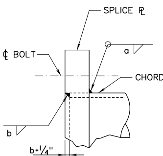
DETAIL 7
