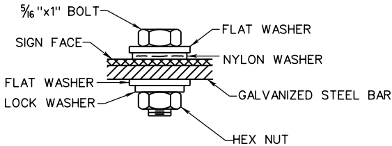
DETAIL 'C'
