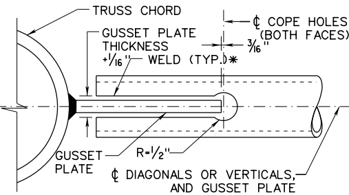
COPING DETAIL
