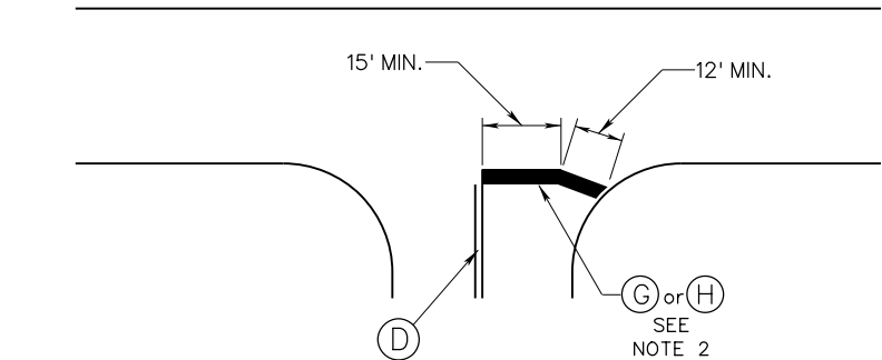
(G) METHODOLOGY FOR INSTALLING (BENDING) STOP LINES AT WIDE THROATED INTERSECTIONS
