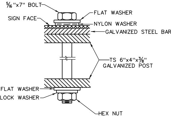
DETAIL 'D'
