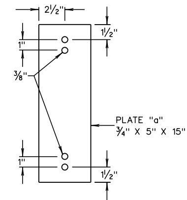
PLATE "a"
