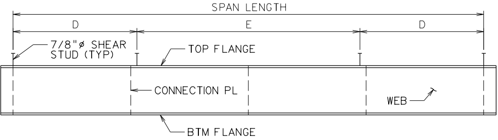
BEAM ELEVATION
