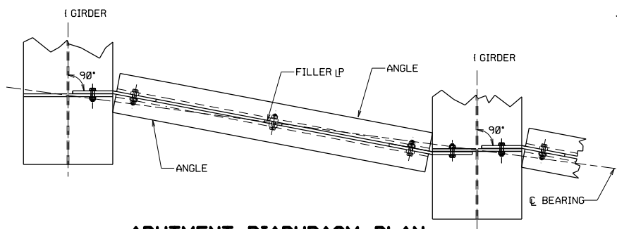
ABUTMENT DIAPHRAGM PLAN
