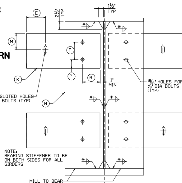
BEARING STIFFENER & CONNECTION PLATES LOOKING AHEAD STATION
