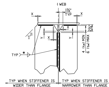
WELDING DETAIL AT END OF STIFFENER X WELD = 1/4" + 1/4" FROM END OF PLATE Y WELD = 1/2" + 1/4" FROM END OF PLATE NOT TO SCALE
