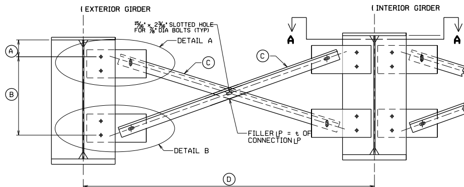
ABUTMENT DIAPHRAGM ELEVATION
