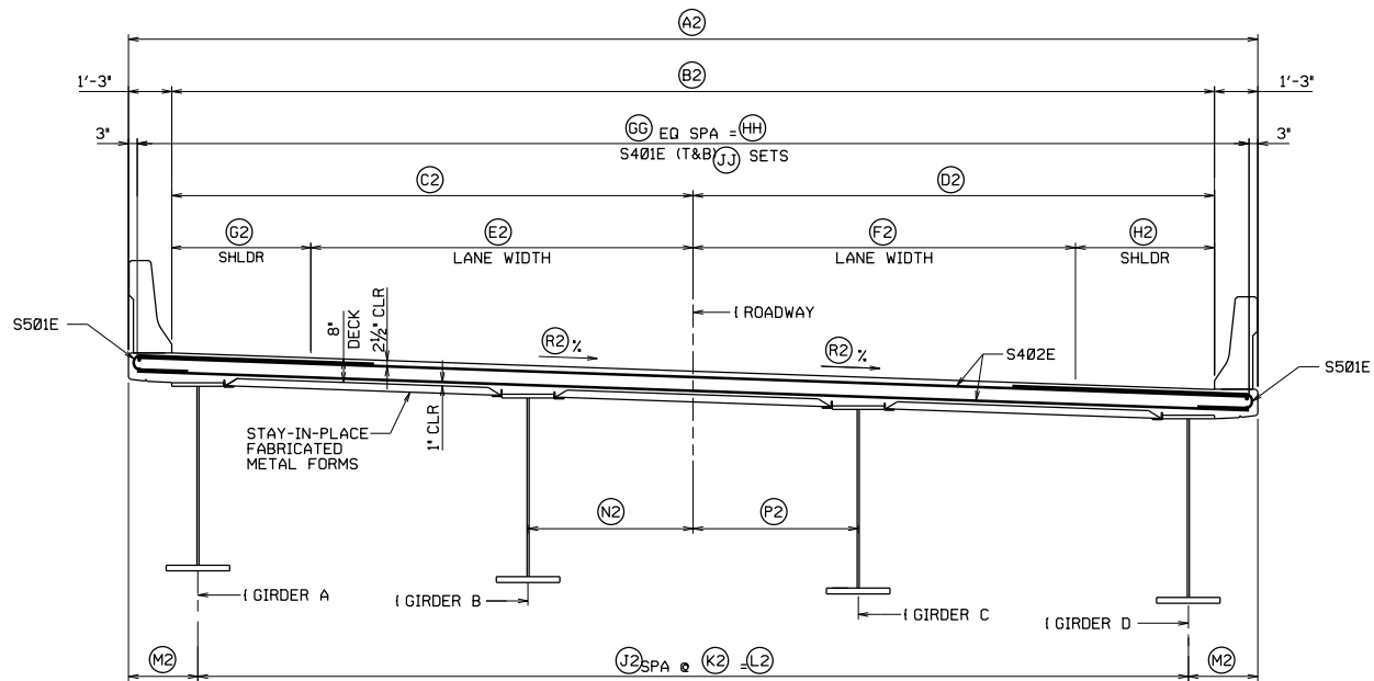
TYPICAL SECTION LOOKING STATION AHEAD
