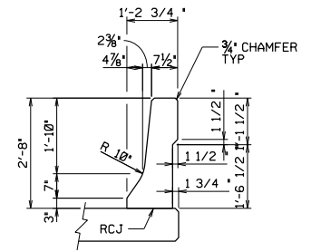
BARRIER DETAIL
