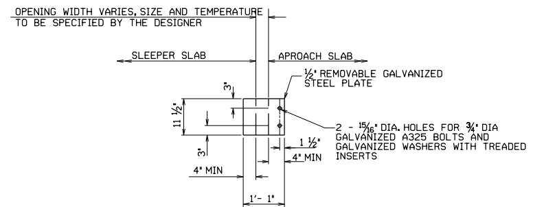
EXPANSION DAM END COVER PLATE
