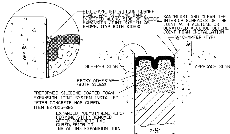
EXPANSION JOINT SEALING DETAIL
