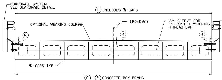
TYPICAL CROSS-SECTION WITH GUARDRAIL
