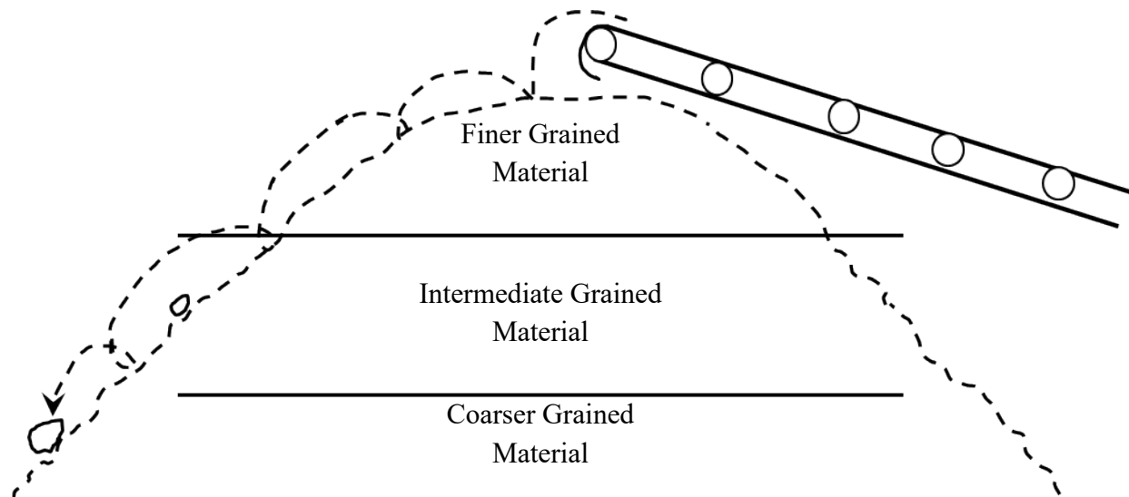
Figure 35 - Stockpile Segregation
