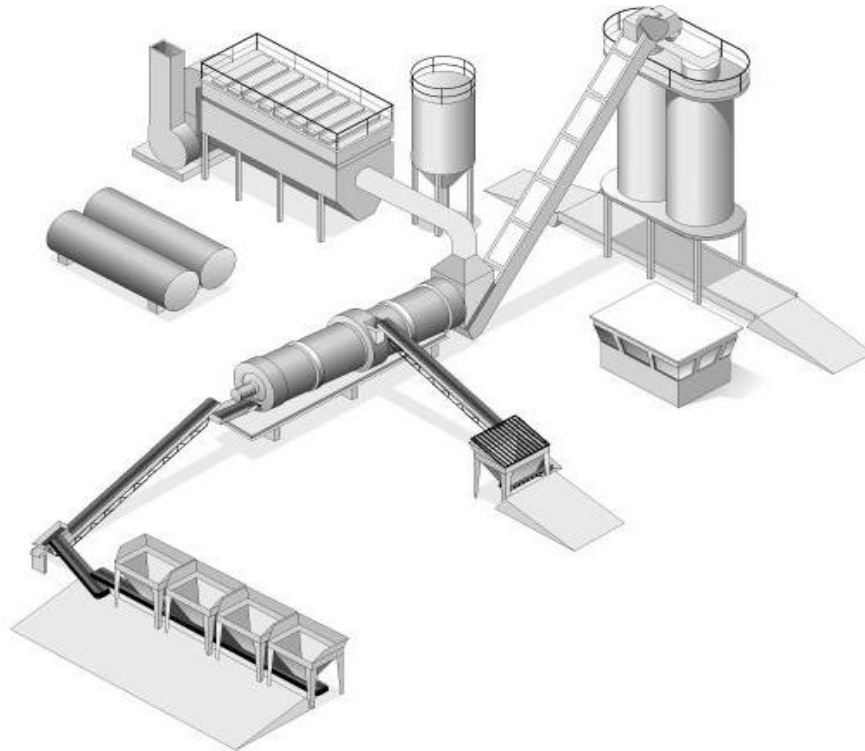
Figure 28 - Drum Mixing Plant
