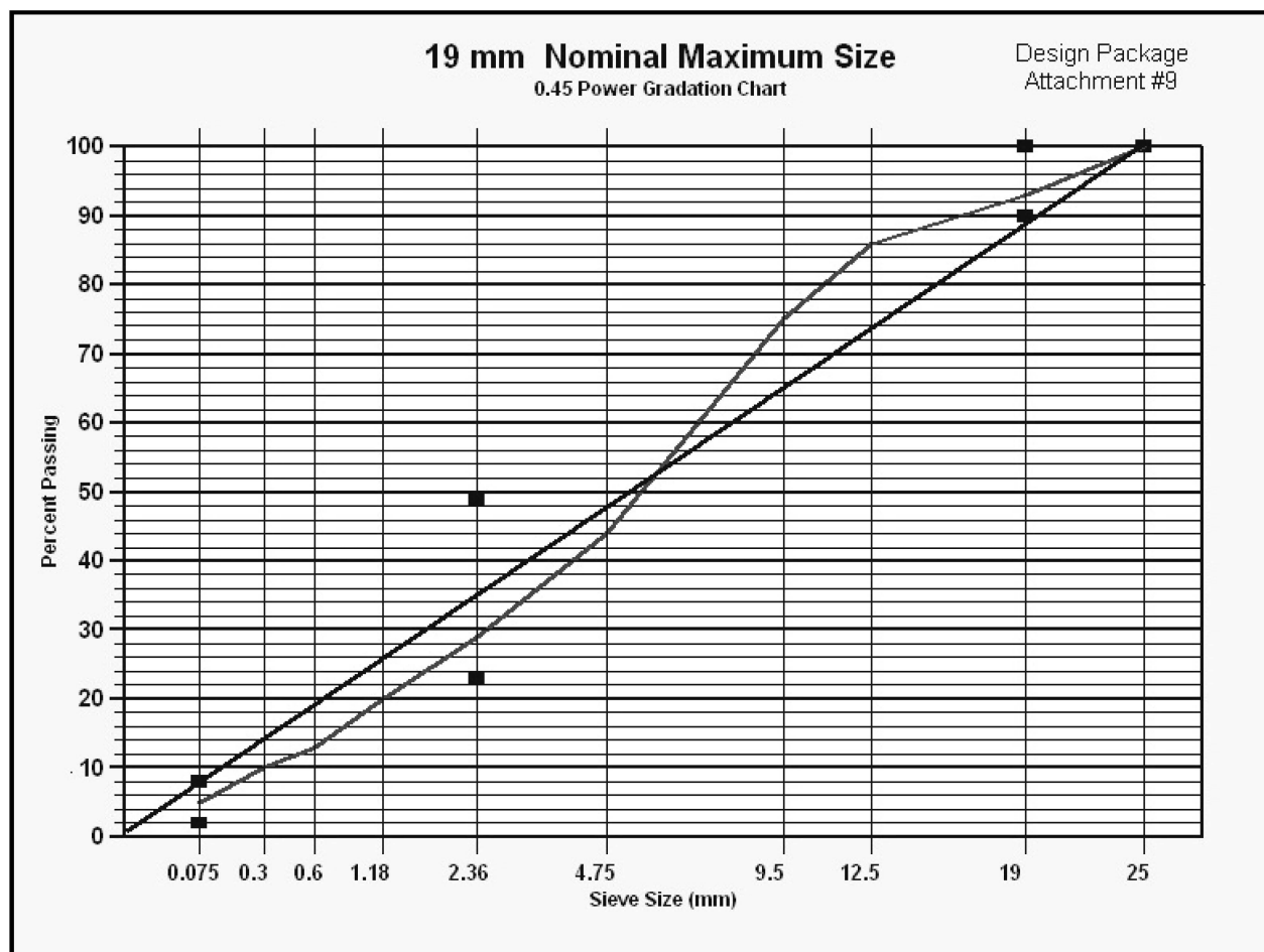
Figure 43 - Power 45 Chart for a 19mm NMA
