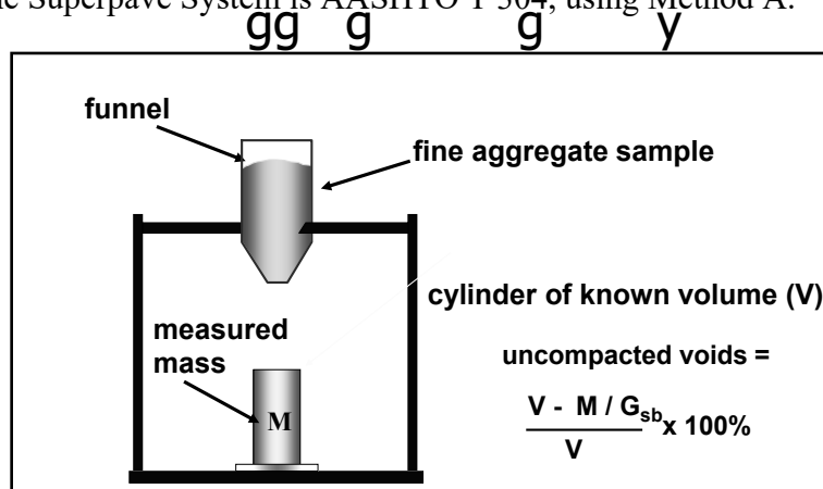
Figure 45 - Fine Aggregate Angularity
