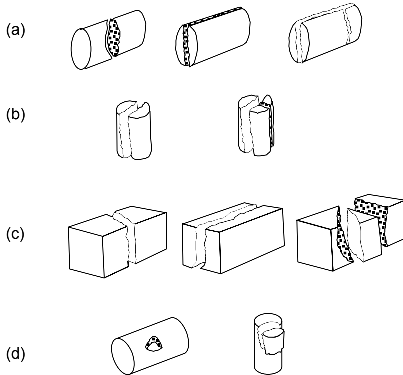
Figure 7: Typical Modes of Failure for Valid and Invalid Tests
