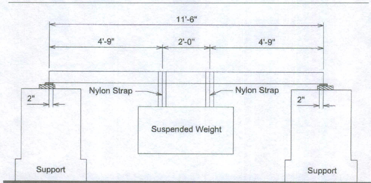
Figure 2. Test Setup
