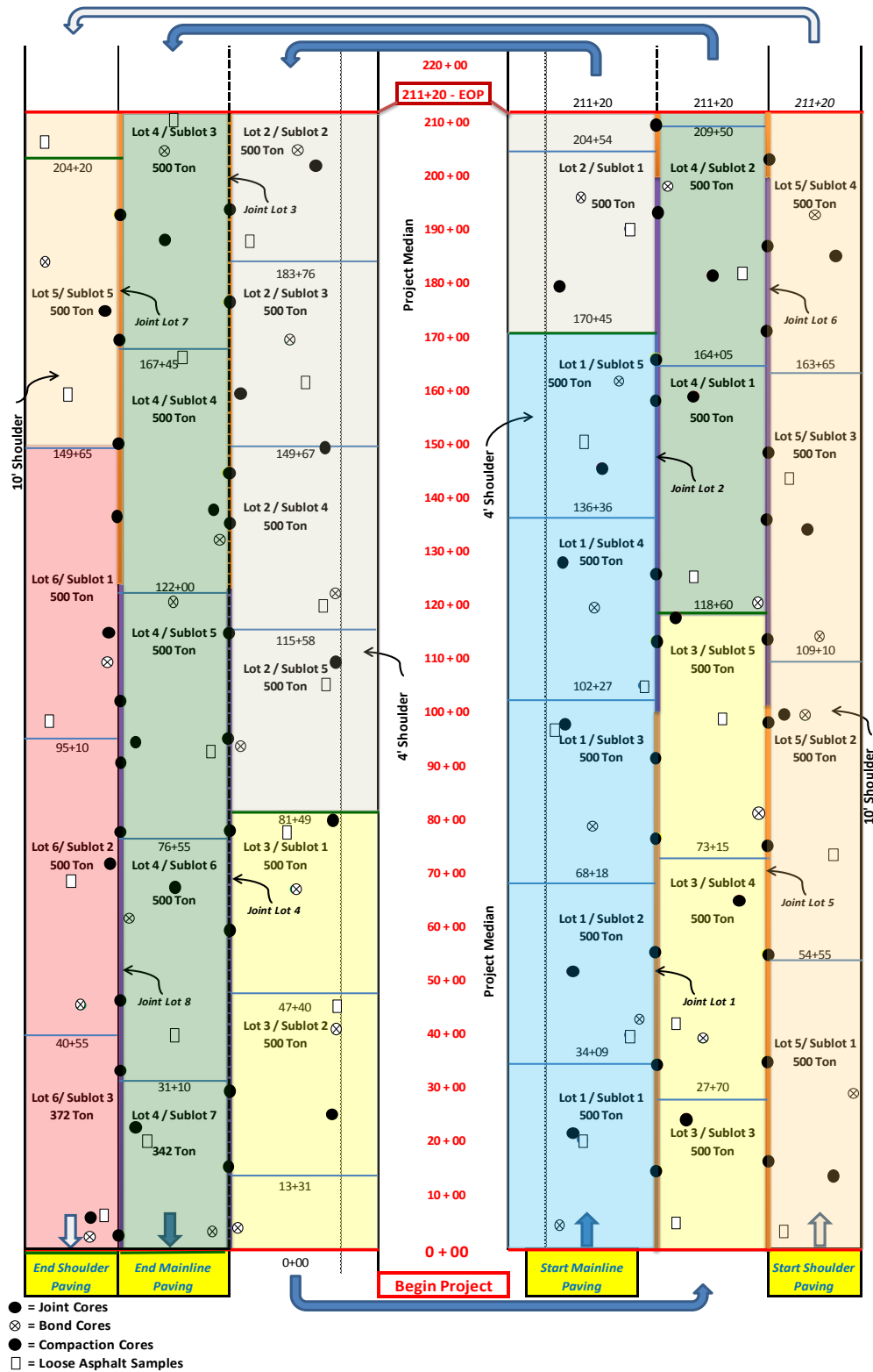
Figure 3 Project Layout with Sampling Plan - Density and Bond Cores, Loose Mix Samples
